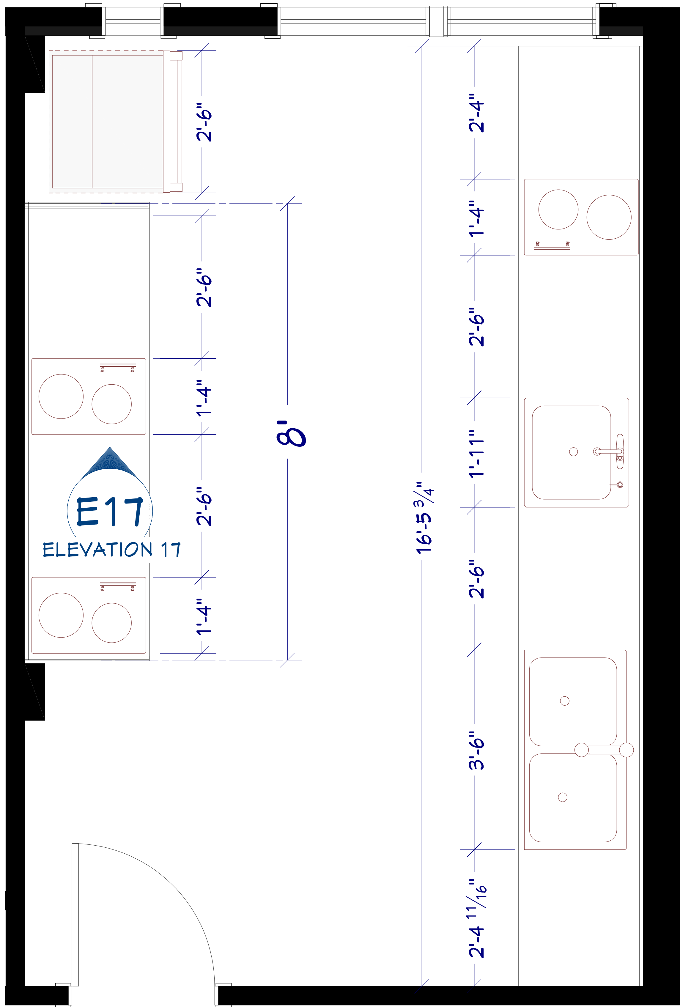
P1 KITCHEN PLAN A14 Scale: 1" = 1'
